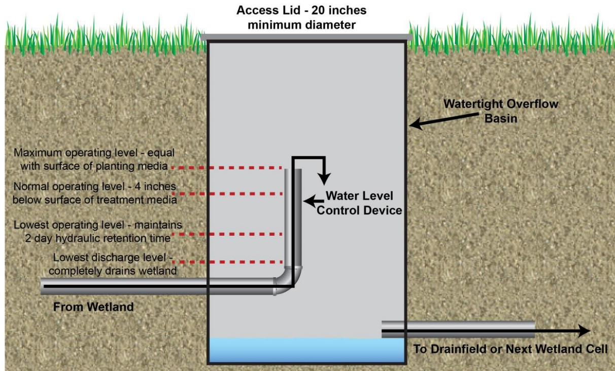
Figure 4-52. Cross-sectional view of an overflow basin.
