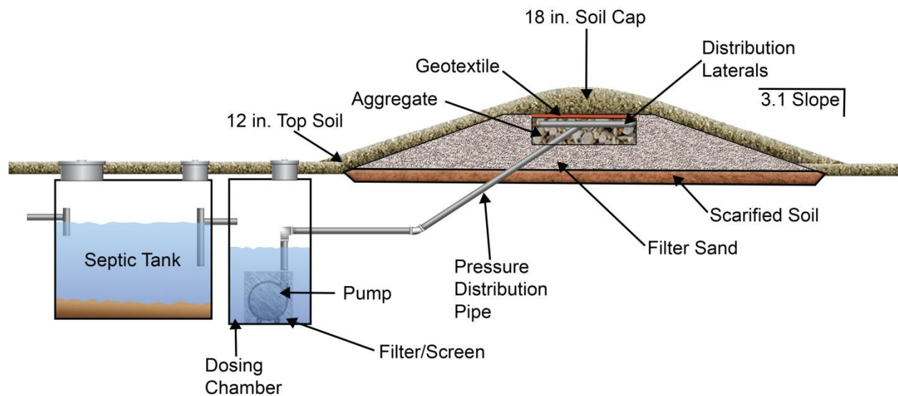
Figure 4-42. Cross-sectional view of sand mound.
